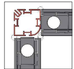
MULTI CORNER POST (CURVE FACING IN, SEG SLOTS FACING OUT)
